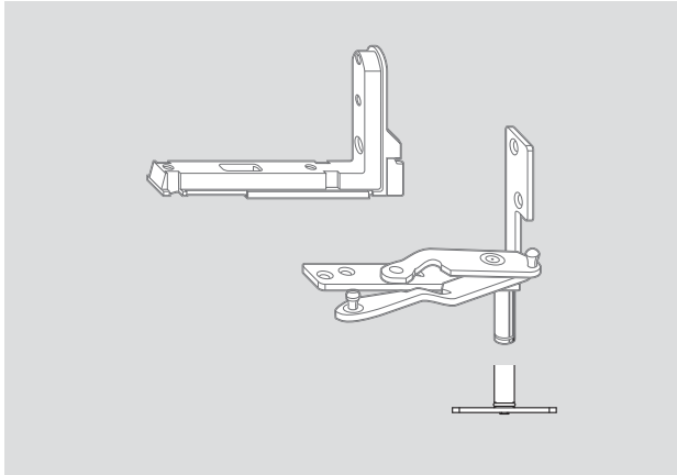
Counter bearing for sash weight 80–130 kg 474138
